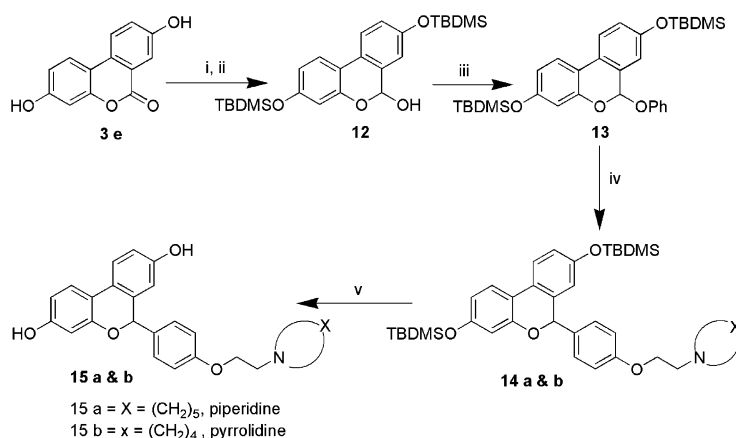
Scheme 4. Reagents and conditions: (i) TBDMSCl, imidazole, DMF, (ii) DIBAL-H, -95 to -75^{\circ}\text{C} , (iii) 4-(2-piperidinoethoxy)/4-(2-pyrrolidinoethoxy) phenyl magnesium bromide, dry THF (v) \text{I}_2 , methanol, rt.
