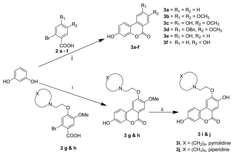
Scheme 1. Reagents and conditions: (i) CuSO 4 /NaOH, heat; (ii) BBr 3 , DCM, –78 °C.
