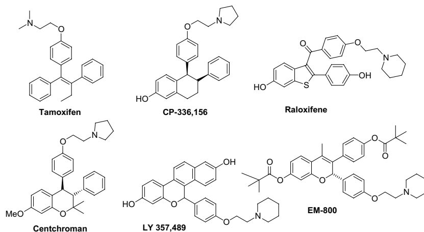
Chart 1. Structures of some potential oestrogen antagonists/SERMs.
