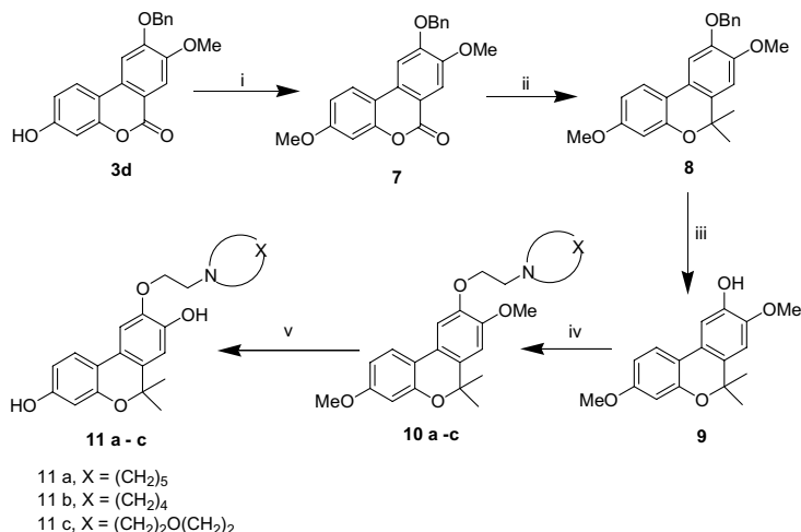
Scheme 3. Reagents and conditions: (i) Methyl iodide, anhyd \text{K}_2\text{CO}_3 , dry acetone, (ii) methyl magnesium iodide, dry ether/dry THF, reflux, (iii) Raney nickel, methanol, \text{H}_2 (60 mm), (iv) 1-(2-chloroethyl) amines, anhyd \text{K}_2\text{CO}_3 , dry acetone, (v) \text{BBr}_3 , DCM, -78^\circ\text{C} .
