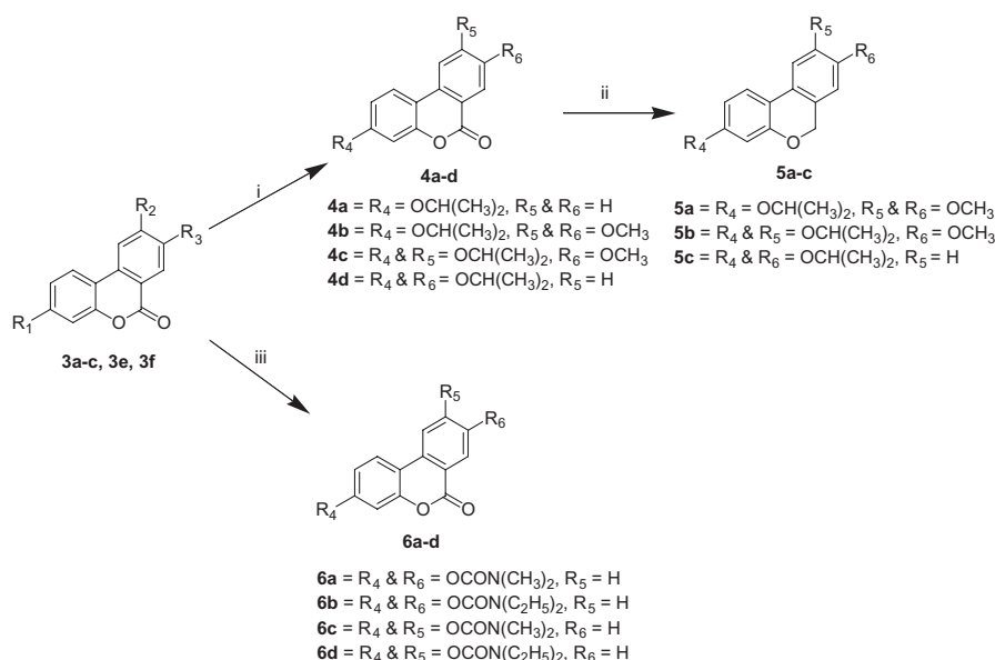
Scheme 2. Reagents and conditions : (i) Isopropyl bromide, anhyd \text{K}_2\text{CO}_3 , dry acetone; (ii) (\text{CH}_3)_2\text{S}\cdot\text{BH}_3 /dry THF; (iii) dimethyl/diethyl carbamoyl chloride, pyridine, rt.
